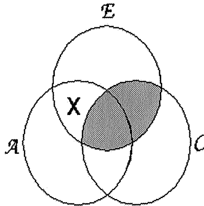
Figure 1. Venn diagram for the existential reconstruction.
