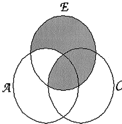
Figure 2. Venn diagram for the universal reconstruction.
